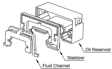
Fig 2.9.4 Cassette Unit
